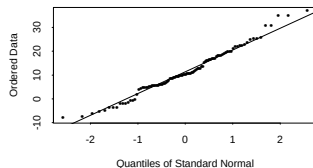
Data from a heavy-tailed distribution
